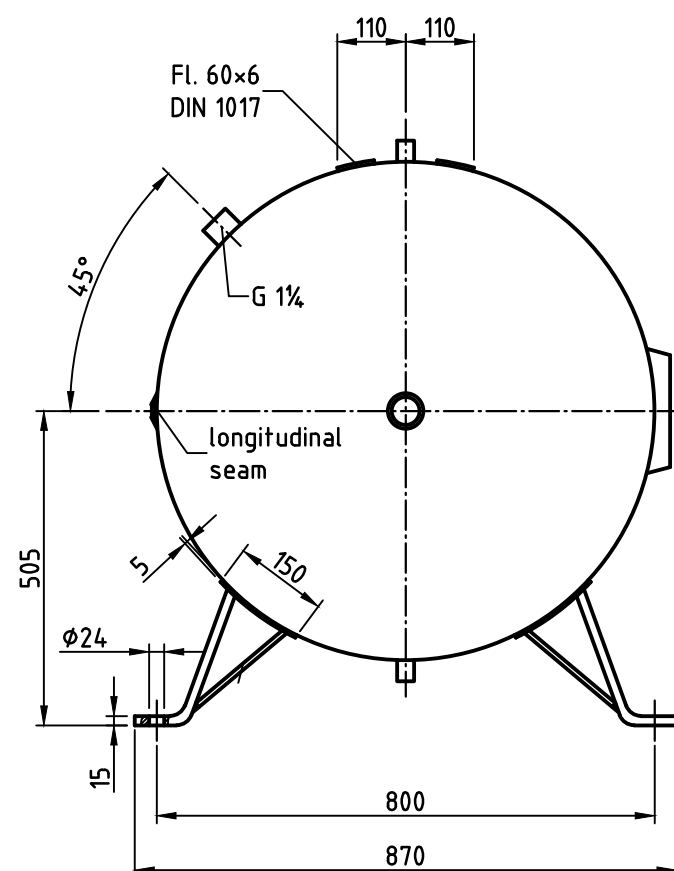
view A
